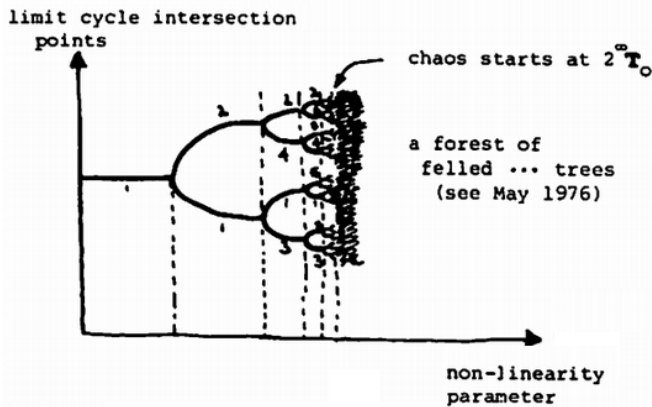
FIG. 3. The period doubling cascade.
